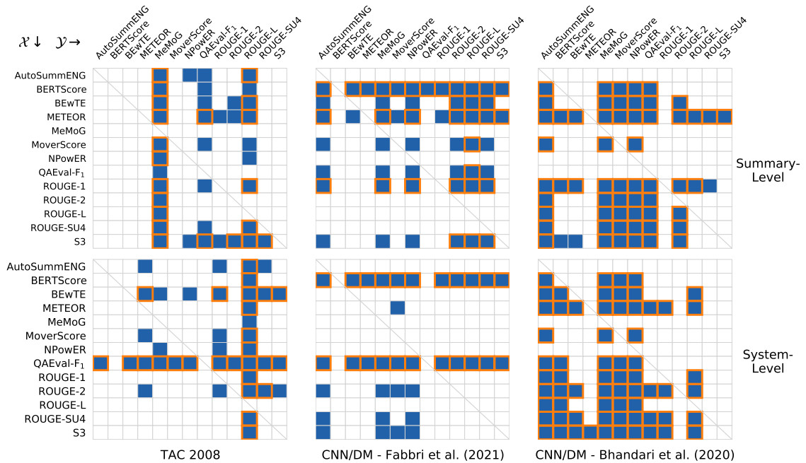
Figure 29: The results of running the PERM-BOTH hypothesis test to find a significant difference between metrics’ Pearson correlations. A blue square means the test returned a significant p -value at \alpha = 0.05 , indicating the row metric has a higher correlation than the column metric. An orange outline means the result remained significant after applying the Bonferroni correction. Summary-level correlations are the top row and system-level on the bottom. TAC 2008 is in the left column, SummEval in the middle, and REALSumm on the right.
