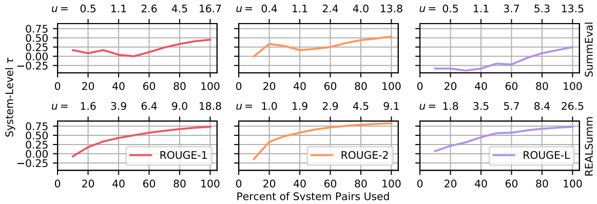
Figure 41: The r_{\text{SYS}}\Delta(\ell, u) correlations on the SummEval (top) and REALSumm (bottom) datasets for \ell = 0 and various values of u for ROUGE-1, ROUGE-2, and ROUGE-L. The u values were chosen to select the 10%, 20%, ..., 100% of the pairs of systems closest in score. Each u is displayed on the top of each plot.
