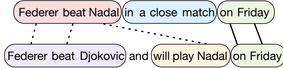
Figure 4: An example token alignment created by ROUGE. Each color represents a summary content unit (SCU) that marks informational content. Only 2/5 of the token alignments (the solid edges) can be explained by matches between phrases that express the same information (the green phrases).
