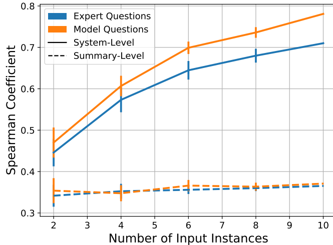
Figure 10: A comparison of the correlations of QAEval- F_1 on a subset of TAC 2008 using expert-written and model-generated questions. Each point represents the average correlation calculated using 30 samples of \{2, 4, 6, 8, 10\} instances, plotted with 95% error bars. System-level correlations were calculated against the summarizers’ average responsiveness scores across the entire TAC 2008 dataset. We hypothesize the model questions perform better due to their verbosity, which causes more keywords to be included in the question that the QA model can match against the summary.
