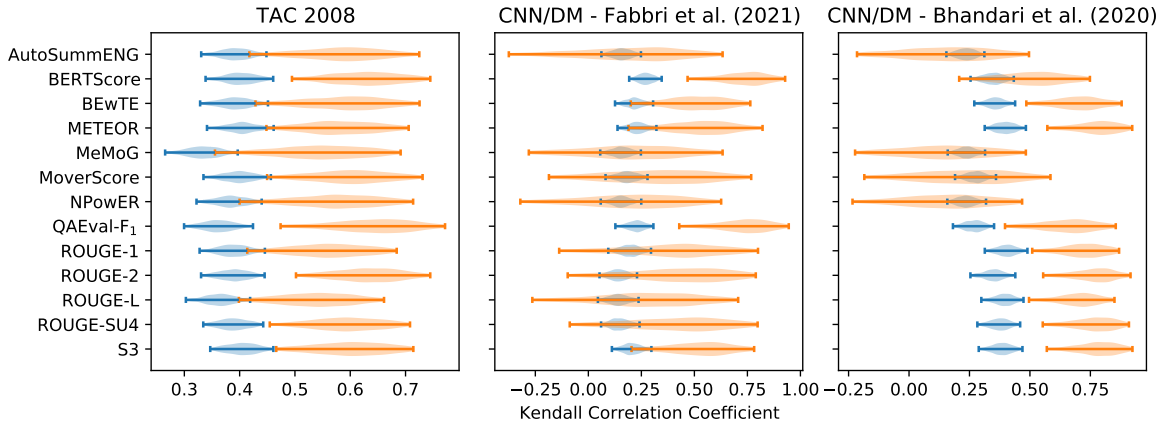
Figure 28: The 95% confidence intervals for \rho_{\text{SUM}} (blue) and \rho_{\text{SYS}} (orange) calculated using Kendall’s correlation coefficient on TAC 2008 (left) and CNN/DM summaries (middle, SummEval; right, REALSumm) are rather large, reflecting the uncertainty about how well these metrics agree with human judgments of summary quality.
