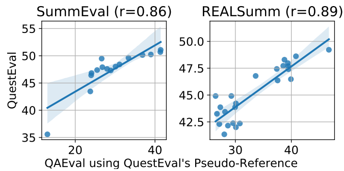
Figure 19: Calculating a system's QA Eval score against the psuedo-reference chosen to maximize its QuestEval score is strongly correlated with that same systems' QuestEval score on SummEval and REALSumm.
