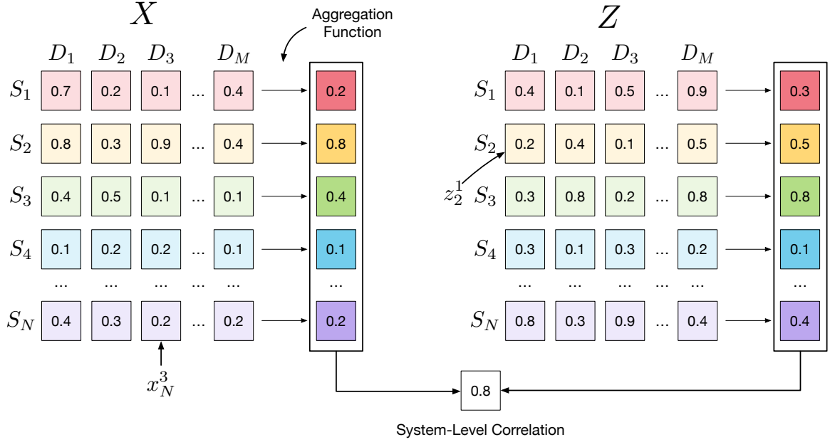
Figure 1: The system-level correlation calculates the correlation between the metric and ground scores for each system, typically calculated by aggregating over the scores per-input.
