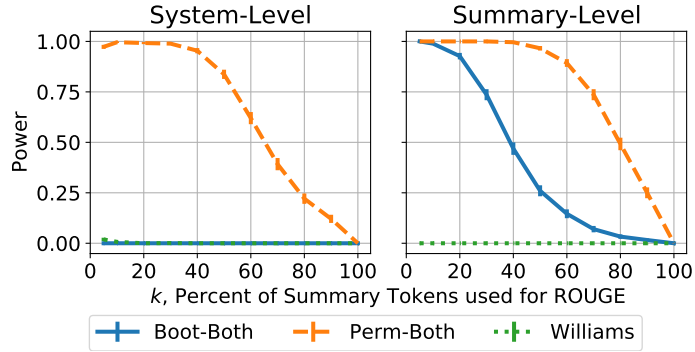
Figure 27: The system- and summary-level Pearson estimates of the power of the BOOT-BOTH, PERM-BOTH, and Williams hypothesis test methods calculated on the annotations from Fabbri et al. (2021). The power for BOOT-BOTH and Williams at the system-level is \approx 0 for all values.
