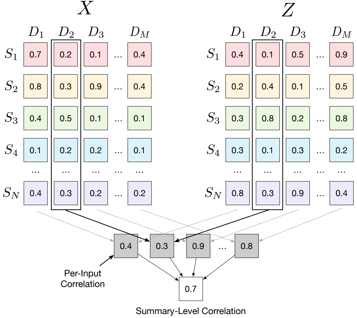
Figure 2: The summary-level correlation calculates the correlation between the metric and ground scores per input, then averages the correlations to calculate the final score.
