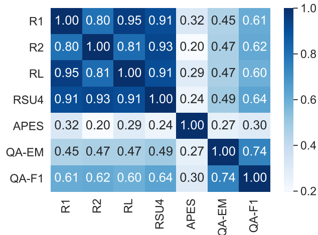
Figure 12: The Pearson correlations between the scores of several ROUGE variants, APES, and QAEval variants on TAC’08. The results support similar findings of Eyal et al. (2019), namely that the ROUGE metrics are highly correlated to each other but have low correlation to the QA-based metrics, suggesting the two types of metrics offer complementary signals.
