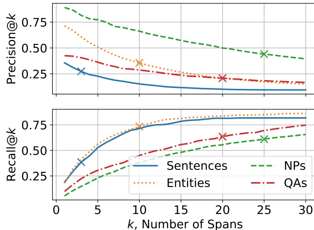
Figure 36: The performances of the salient span classifiers using the different types of salient phrase labeling evaluated against the silver spans. The “x” marks the operating points used in the end-to-end models.
