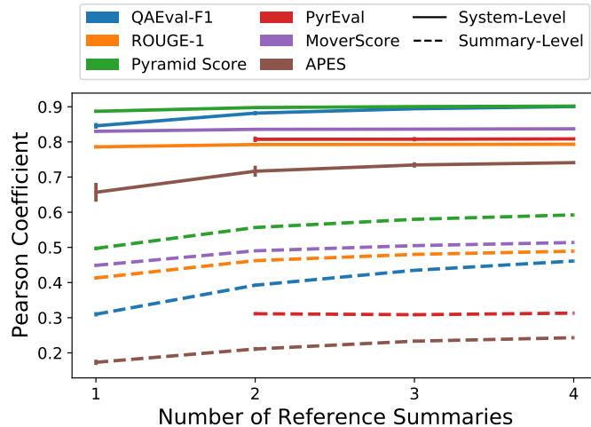
Figure 35: The system- and summary-level Pearson correlations as the number of available reference summaries increases. 95% confidence error bars shown, but may be too small to see. PyEval is missing data because the official implementation requires at least two references. Even with one reference summary, QAEval-F 1 maintains a higher system-level correlation than ROUGE.
