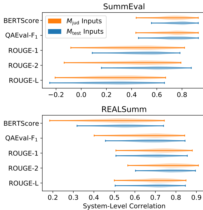
Figure 40: The 95% CIs calculated using the BOOT-BOTH bootstrapping method with M_{jud} summaries in orange and M_{test} in blue.
