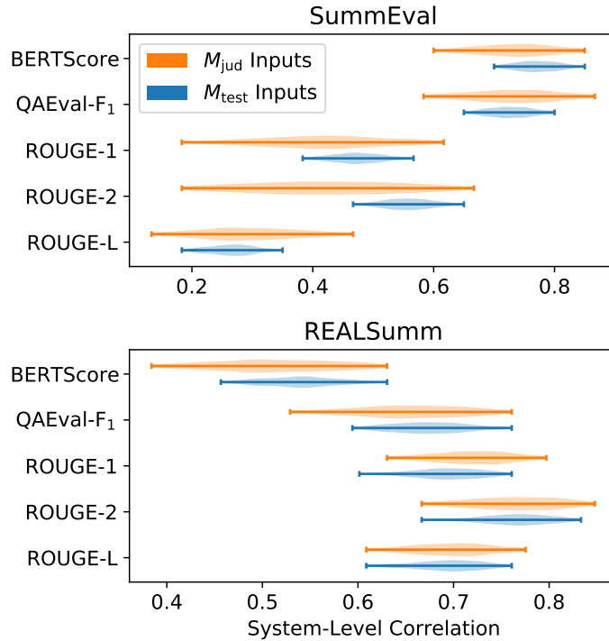
Figure 32: 95% confidence intervals for r_{\text{SYS}} calculated with the BOOT-INPUTS resampling method when the system rankings for the automatic metrics are calculated using only the judged data (orange) versus the entire test set (blue). Scoring systems with more summaries leads to better (more narrow) estimates of r_{\text{SYS}} .
