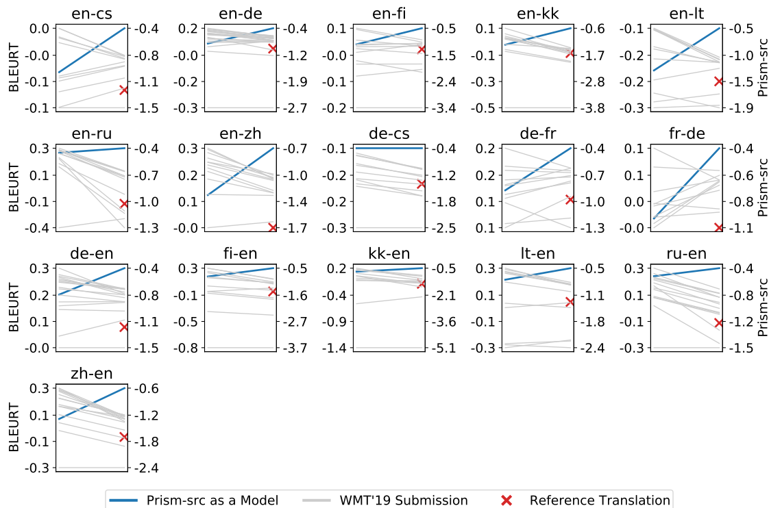
Figure 14: Directly optimizing Prism-src (blue line; §5.4.1) yields the highest Prism-src performance (right y-axis) but only an average system as evaluated by BLEURT (left y-axis). The reference translation (red “x”) has a lower Prism-src score compared to many systems across all language pairs, demonstrating Prism-src’s biases toward learned model output and against human-written translations.
