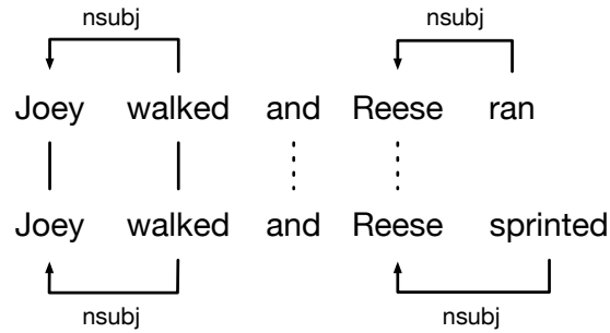
Figure 7: The VB+NSUBJ category selects tuples of verbs and their corresponding NSUBJ dependents in the dependency tree. In this example, 2/4 of the alignment (the solid lines) can be explained by matches between such tuples. The dashed lines cannot: The “and” alignment is not part of any tuple; Since “ran” and “sprinted” are not aligned, their corresponding tuples are not considered to be aligned, so the “Reese” match does not count toward the total.
