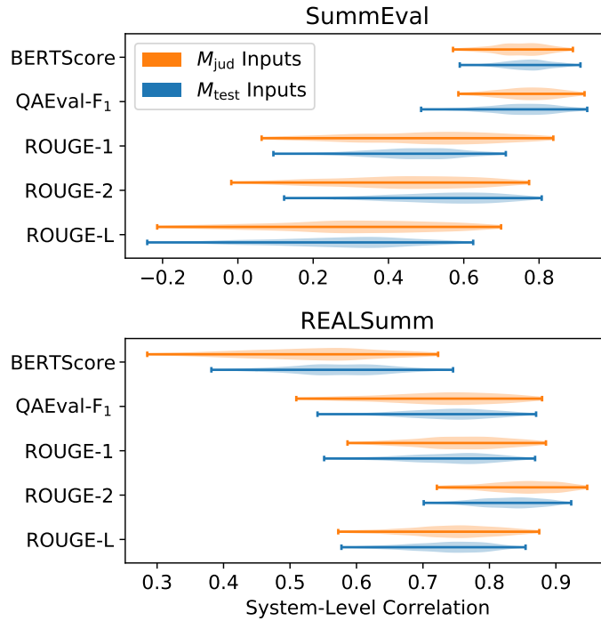
Figure 39: The 95% CIs calculated using the BOOT-SYSTEMS bootstrapping method with M_{jud} summaries in orange and M_{test} in blue.
