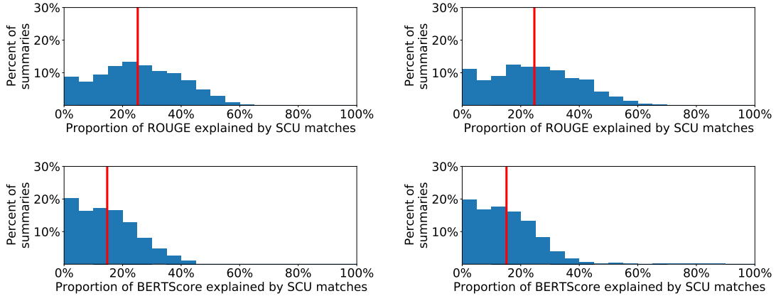
Figure 5: The distribution of the proportion of ROUGE (top row) and BERTScore (bottom row) on TAC 2008 (left column) and TAC 2009 (right column) that can be explained by tokens matches that are labeled with the same SCU (Eq. 3.5). The averages, around 25% and 15% on both datasets (in red), indicate that only a small amount of their scores is between phrases that express the same information.
