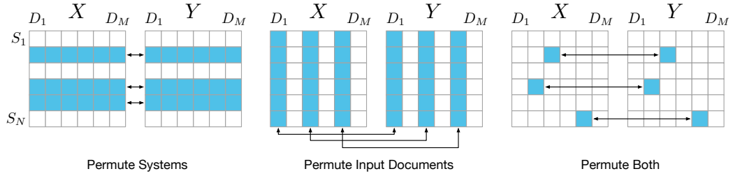
Figure 26: An illustration of the three permutation methods which swap system scores, document scores, or scores for individual summaries between X and Y .
