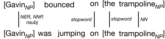
Figure 6: Every token alignment used by ROUGE or BERTScore is assigned to one or more interpretable categories (defined in §3.5). This allows us to calculate, for this example, that matches between named-entities contribute 1/4 to the overall score, stopwords 2/4, and noun phrases 3/4 (assuming alignment weights of 1.0).
