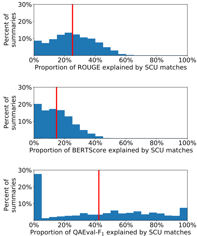
Figure 13: The distribution of the proportion of the ROUGE (top), BERTScore (middle), and QAEval-F 1 (bottom) scores that can be explained by SCU matches on TAC 2008 (top two plots taken from Fig. 5). Although its variance is higher, we find that QAEval can be explained by SCU matches far more than ROUGE or BERTScore on average.
