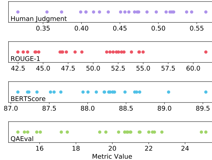
Figure 33: The systems (each represented by a point) on the two datasets (shown here for REAL-Summ) are rather diverse in quality as measured by both human judgments and automatic metrics.
