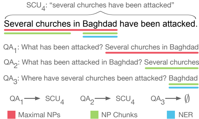
Figure 8: Example answers selected by the three strategies. The only SCU marked by annotators for this sentence is SCU 4 , which does not include information about the location of the attacks. Therefore, an answer selection strategy that chooses “Baghdad” enables generating a QA pair such as QA 3 , which probes for information not included in the Pyramid annotation.
