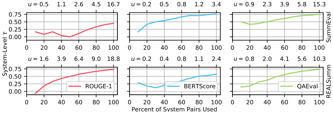
Figure 34: The r_{\text{SYS}}\Delta(\ell, u) correlations on the SummEval (top) and REALSumm (bottom) datasets for \ell = 0 and various values of u (additional combinations of \ell and u can be found in Appendix D.2). The u values were chosen to select the 10%, 20%, ..., 100% of the pairs of systems closest in score. Each u is displayed on the top of each plot. For instance, 20% of the \binom{N}{2} system pairs on SummEval are separated by < 0.5 ROUGE-1, and the system-level correlation on those pairs is around 0.08. As more systems are used in the correlation calculation, the allowable gap in scores between system pairs increases, and are therefore likely easier to rank, resulting in higher correlations.
