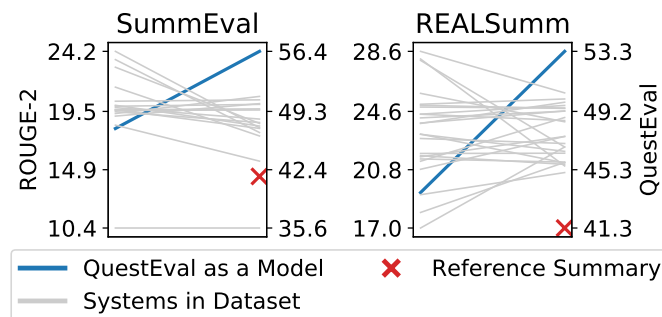
Figure 16: Nearly all models in the SummEval and REALSumm datasets have better QuestEval scores than the reference summaries, demonstrating the metrics bias toward learned model output over human-written text.
