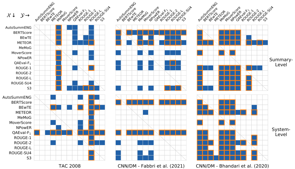
Figure 38: The results of running the PERM-BOTH hypothesis test to find a significant difference between metrics’ Pearson correlations with the Bonferroni correction applied per dataset and correlation level pair instead of per metric (as in Fig. 29). A blue square means the test returned a significant p -value at \alpha = 0.05 , indicating the row metric has a higher correlation than the column metric. An orange outline means the result remained significant after applying the Bonferroni correction.
