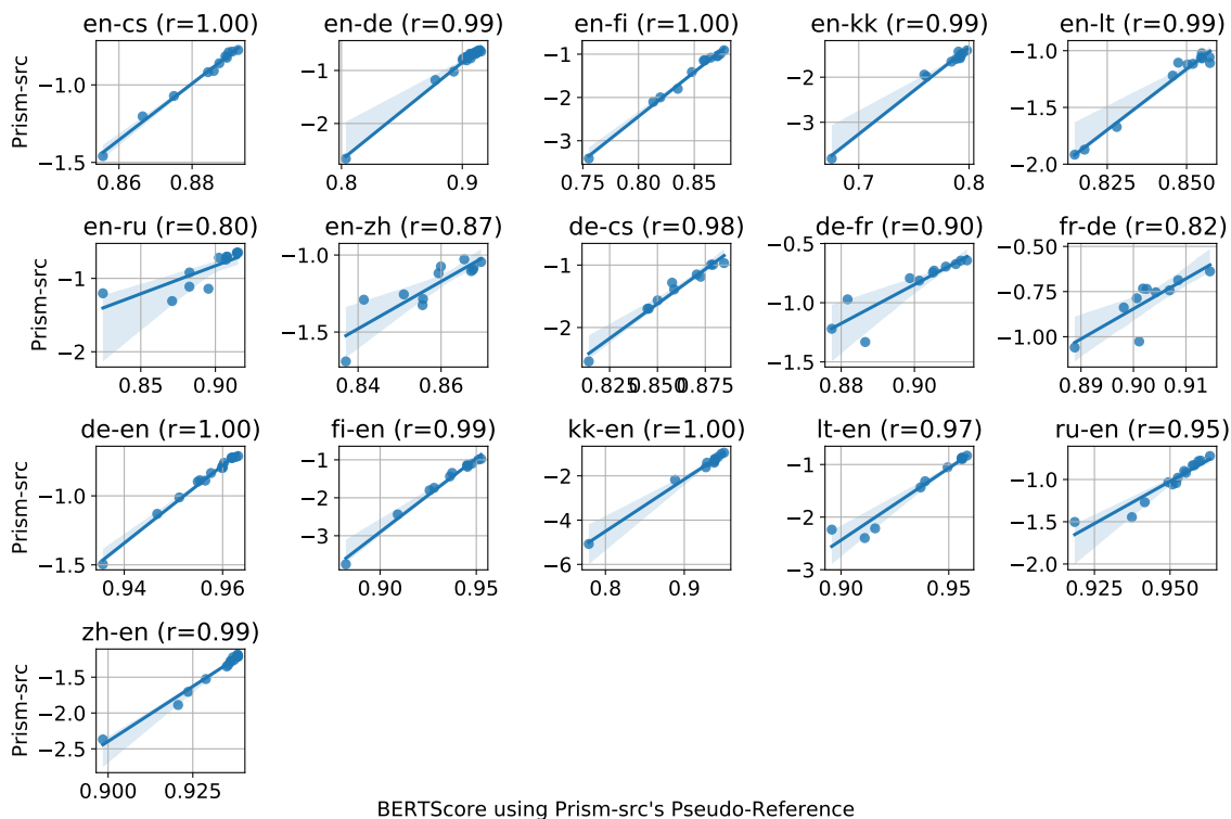
Figure 17: A system’s BERTScore in which the output from directly optimizing Prism-src is used as the reference (x-axis) is strongly correlated to that same system’s Prism-src score (y-axis). This demonstrates Prism-src is roughly equivalent to evaluating systems with a pseudo-reference translation which is generated by a model. Pearson’s r shown in the title of each plot.
