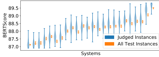
Figure 30: The bootstrapped 95% confidence intervals for the BERTScore of each system in the REALSumm dataset using M_{\text{jud}} judged instances in blue and M_{\text{test}} instances in orange. Evaluating systems with M_{\text{test}} instances leads to far better estimate of their true scores.
