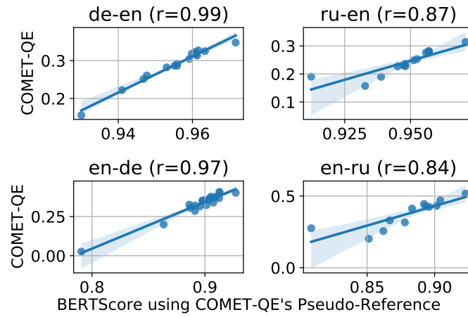
Figure 18: Scoring systems with BERTScore against psuedo-references obtained by optimizing COMET-src strongly correlates to the systems' COMET-src scores.
