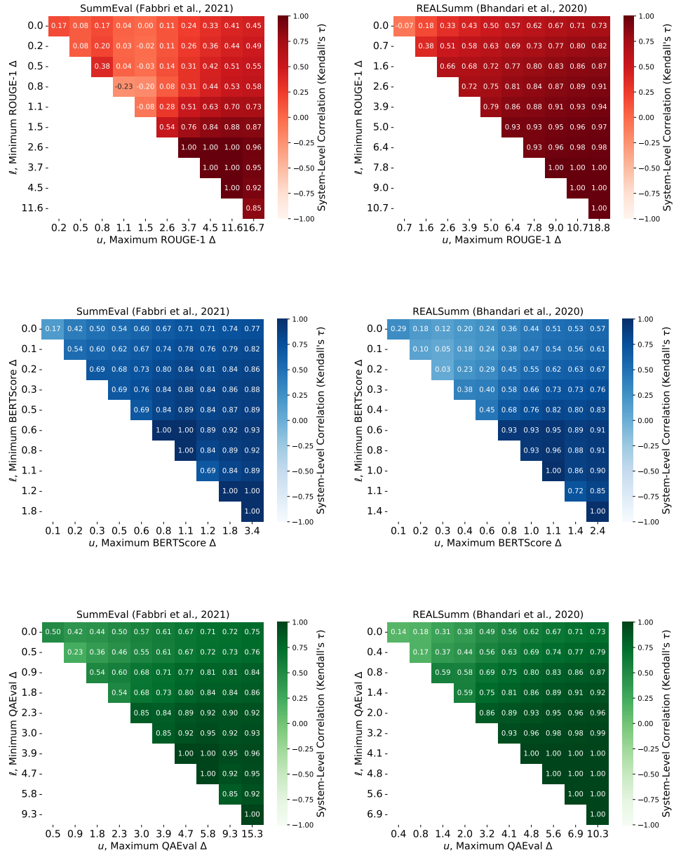
Figure 42: r_{\text{SYS}}\Delta(\ell, u) correlations for various combinations of \ell and u (see §8.4.2) for ROUGE (top), BERTScore (middle), and QAEval (bottom) on SummEval (left) and REALSumm (right). The values of \ell and u were chosen so that each value in the heatmaps evaluates on 10% more system pairs than the value to its left. For instance, the first row evaluates on 10%, 20%, ..., 100% of the system pairs. The second row evaluates on 10%, 20%, ..., 90% of the system pairs, never including the 10% of pairs which are closest in score. The first row of each of the heatmaps is plotted in Fig. 34. The correlations on realistic score differences between systems are in the upper left portion of the heatmaps and contain the lowest correlations overall. Evaluating on all pairs is the top-rightmost entry, and the “easiest” pairs (those separated by a large score margin) are in the bottom right.
