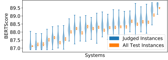
Figure 2: The bootstrapped 95% confidence intervals for the BERTScore of each system in the REALSumm dataset using M_{\text{jud}} judged instances in blue and M_{\text{test}} instances in orange. Evaluating systems with M_{\text{test}} instances leads to far better estimate of their true scores.
