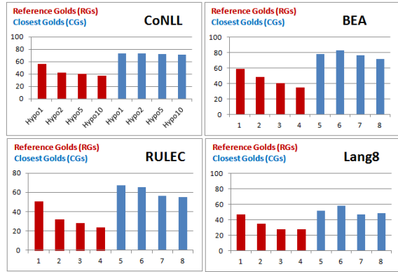
Figure 2: Performance by hypothesis rank (F-score) against Reference Gold (RG) vs. Closest Golds (CGs) generated specially for each hypothesis. Observe dramatic drop in performance between top hypothesis and the rest in RG evaluation, vs. stability in CG evaluation; and large gaps between scores even for the top hypotheses in RG vs. CG evaluations.
